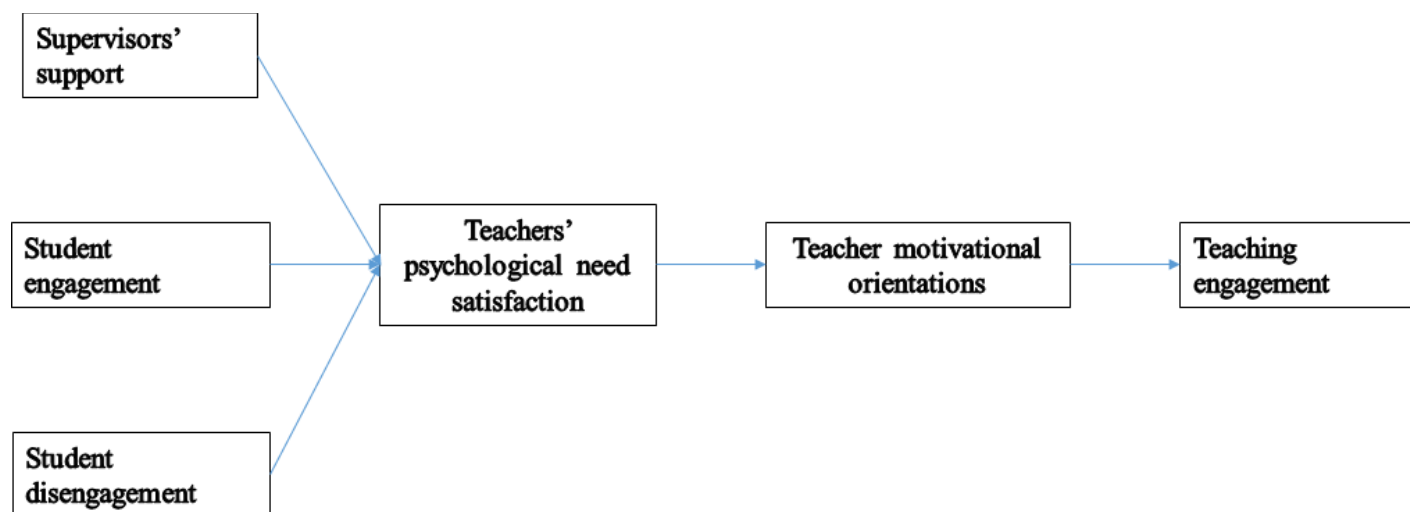
Figure 2. Hypothesized Model
