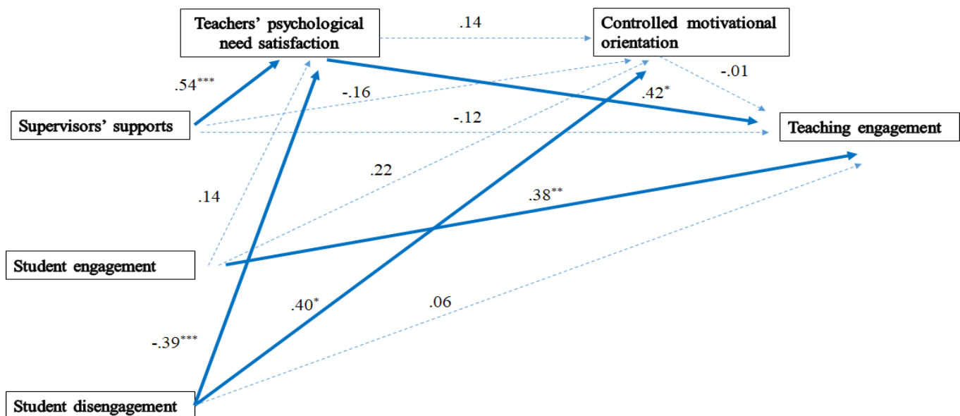
Figure 4. Schematized Results of Path Analyses for the Controlled Motivational Orientation Model
