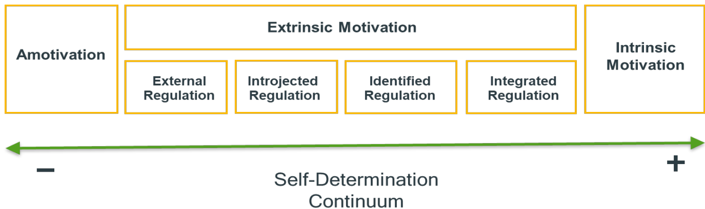
Figure 1. Self-Determination Continuum of Motivation (Adapted from Ryan & Deci, 2017)
