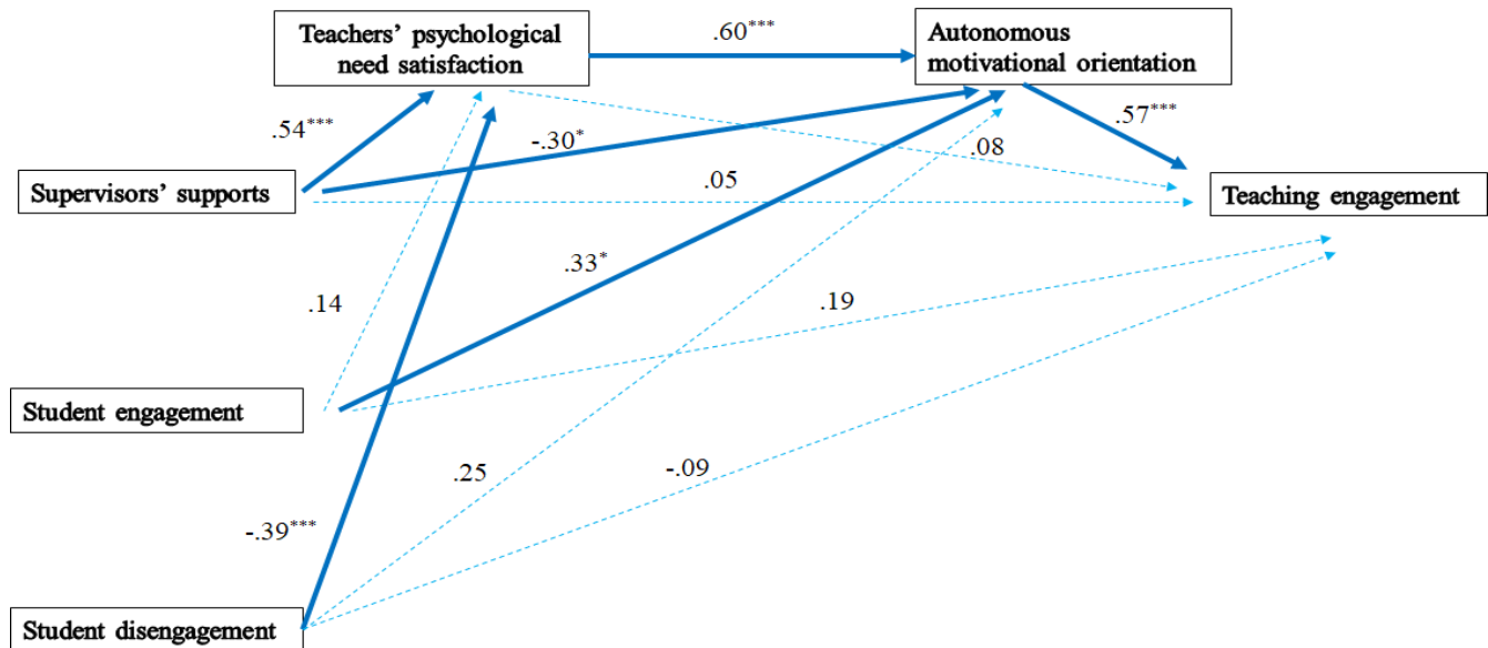
Figure 3. Schematized Results of Regression Analyses for the Autonomous Motivational Orientation Model
